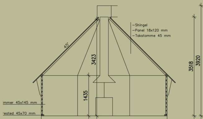
SECTION 1:50
